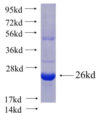
Recombinant Arabidopsis thaliana ANAC19 SDS-PAGE
