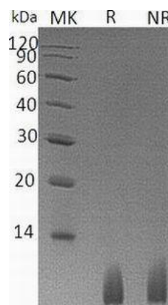
Human UBB (GST & His tag) recombinant protein
