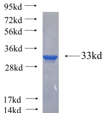
Recombinant human SOX2 SDS-PAGE
