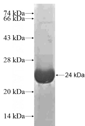
Recombinant Human SLC26A4 SDS-PAGE
