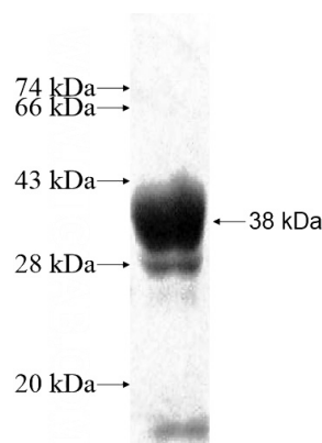
Recombinant Human TSGA13 SDS-PAGE
