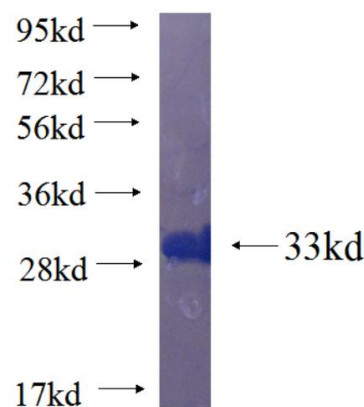
Recombinant human GPM6B SDS-PAGE
