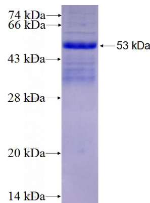
Recombinant Human PDLIM5 SDS-PAGE
