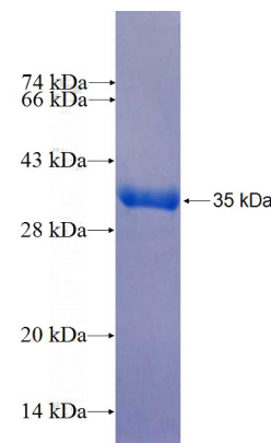
Recombinant Human AGAP3 SDS-PAGE
