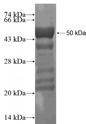
Recombinant Human KDM2A SDS-PAGE
