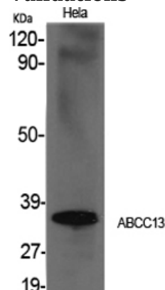
Fig1.; Western Blot analysis of various cells using ABCC13 Polyclonal Antibody cells nucleus extracted by Minute TM Cytoplasmic and Nuclear Fractionation kit (SC-003, Inventibiotec, MN, USA).
