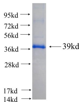
Recombinant human P4HA1 SDS-PAGE
