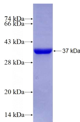
Recombinant Human UPF1 SDS-PAGE
