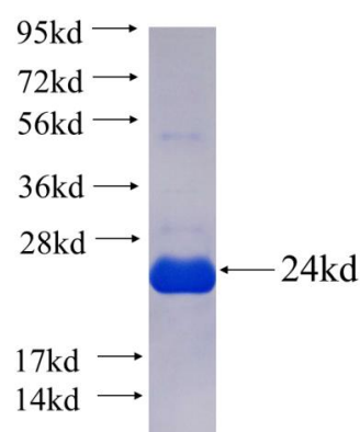
Recombinant human TAF12(Full length) SDS-PAGE
