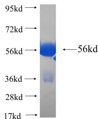
Recombinant Arabidopsis thaliana RGLG1 SDS-PAGE
