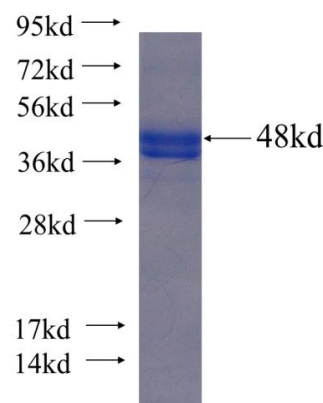
Recombinant Arabidopsis thaliana AtGAP1 SDS-PAGE
