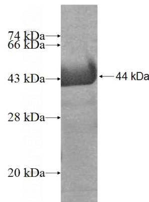
Recombinant Human NRD1 SDS-PAGE
