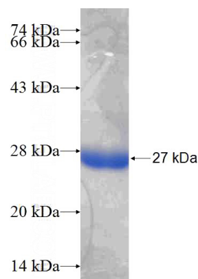
Recombinant Human RANBP3 SDS-PAGE
