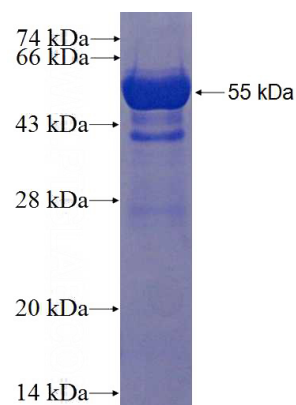
Recombinant Human IRAK1BP1 SDS-PAGE
