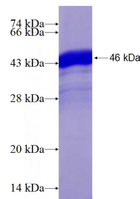
Recombinant Human MYD88 SDS-PAGE
