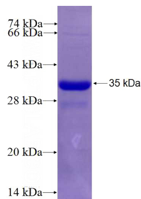
Recombinant Human ABCB6 SDS-PAGE
