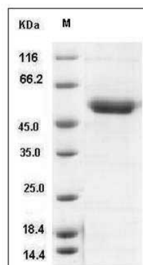
Mouse CD39 / ENTPD1 Protein (His Tag) SDS-PAGE
