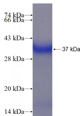
Recombinant Human TOR1A SDS-PAGE
