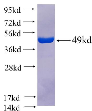
Recombinant Arabidopsis thaliana SQD1 SDS-PAGE
