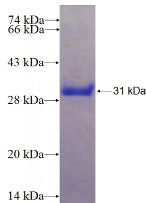
Recombinant Human SUNC1 SDS-PAGE
