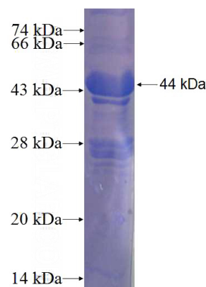
Recombinant Human ROR2 SDS-PAGE
