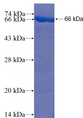
Recombinant Human AHSA1 SDS-PAGE
