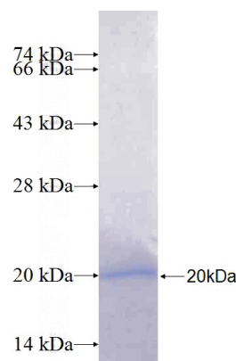
Recombinant Human PRKCQ SDS-PAGE
