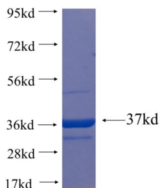
Recombinant Arabidopsis thaliana HDT4 SDS-PAGE
