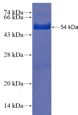
Recombinant Human THEM5 SDS-PAGE
