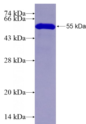
Recombinant Human CDC2L1 SDS-PAGE
