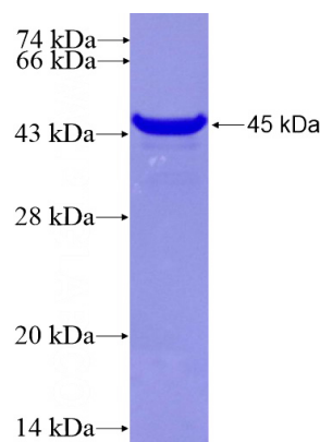
Recombinant Human RANBP10 SDS-PAGE
