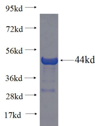
Recombinant human TTC28 SDS-PAGE
