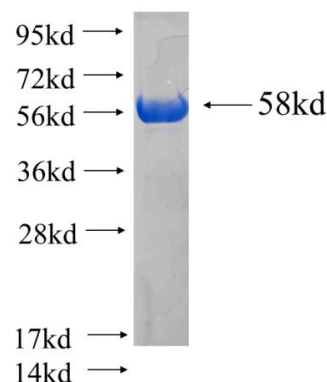
Recombinant human Calretinin SDS-PAGE
