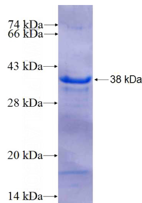
Recombinant Human MYOZ1 SDS-PAGE
