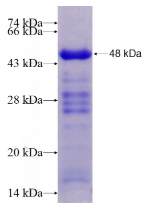
Recombinant Human IDH3B SDS-PAGE
