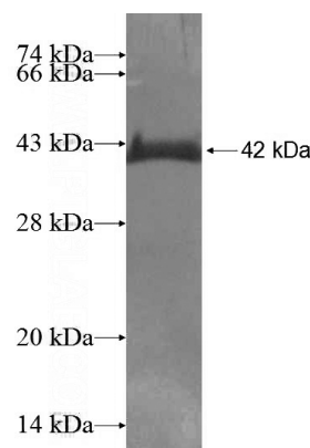
Recombinant Human PSMD5 SDS-PAGE
