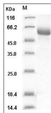
Influenza B (B/Florida/4/2006) Hemagglutinin Protein (HA2 Subunit) (Fc Tag) SDS-PAGE
