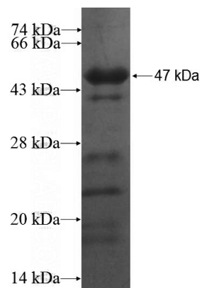
Recombinant Human CCNK SDS-PAGE
