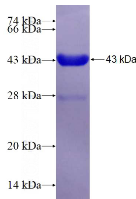
Recombinant Human HSPB6 SDS-PAGE
