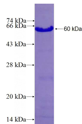
Recombinant Human NAF1 SDS-PAGE
