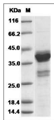
Human MKI67 Protein (GST Tag) SDS-PAGE
