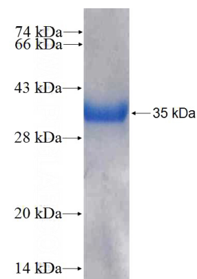
Recombinant Human RAB5B SDS-PAGE
