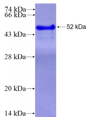
Recombinant Human VGF SDS-PAGE
