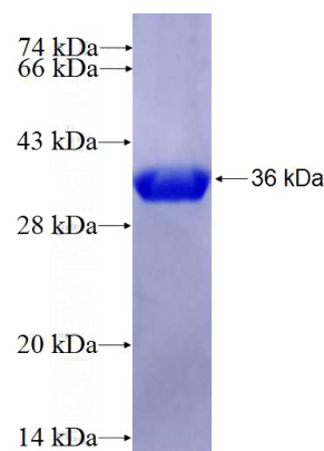
Recombinant Human CKS1B SDS-PAGE
