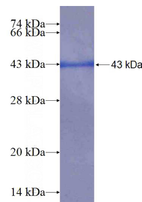
Recombinant Human ADH4 SDS-PAGE
