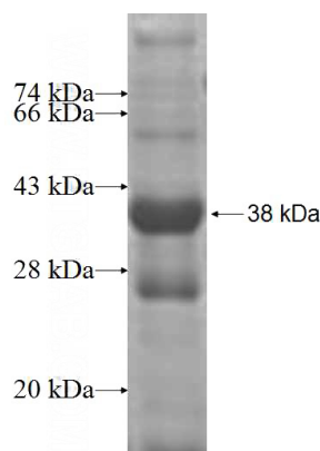
Recombinant Human ATP6V1B1 SDS-PAGE
