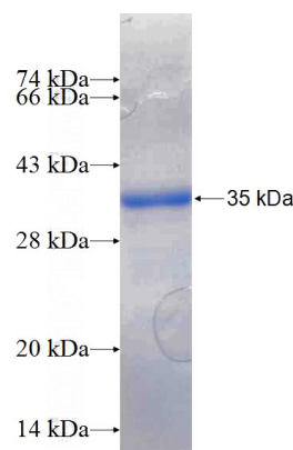
Recombinant Human PANK3 SDS-PAGE
