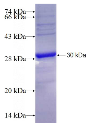
Recombinant Human GABRD SDS-PAGE
