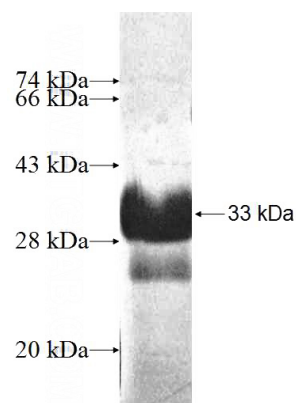
Recombinant Human TSR2 SDS-PAGE
