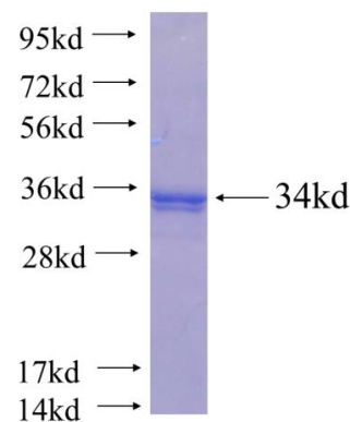
Recombinant Arabidopsis thaliana SHM2 SDS-PAGE
